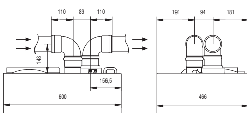
Duo-tec Compact
