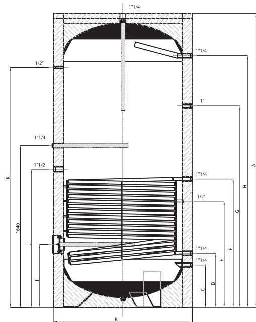
UB 3000 SC
