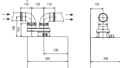
Duo-tec Compact
