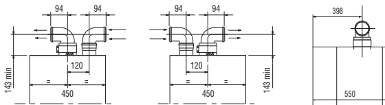
LUNA Duo-tec
